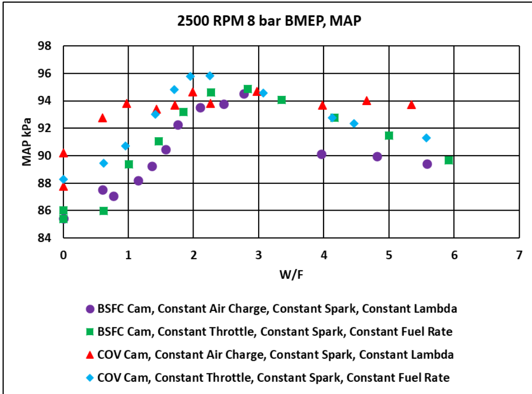
Figure 40 2500 RPM test point atomized spray MAP plot
