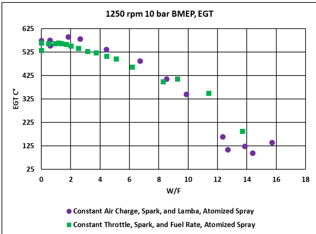
Figure 32 1250 RPM test point atomized spray EGT plot
