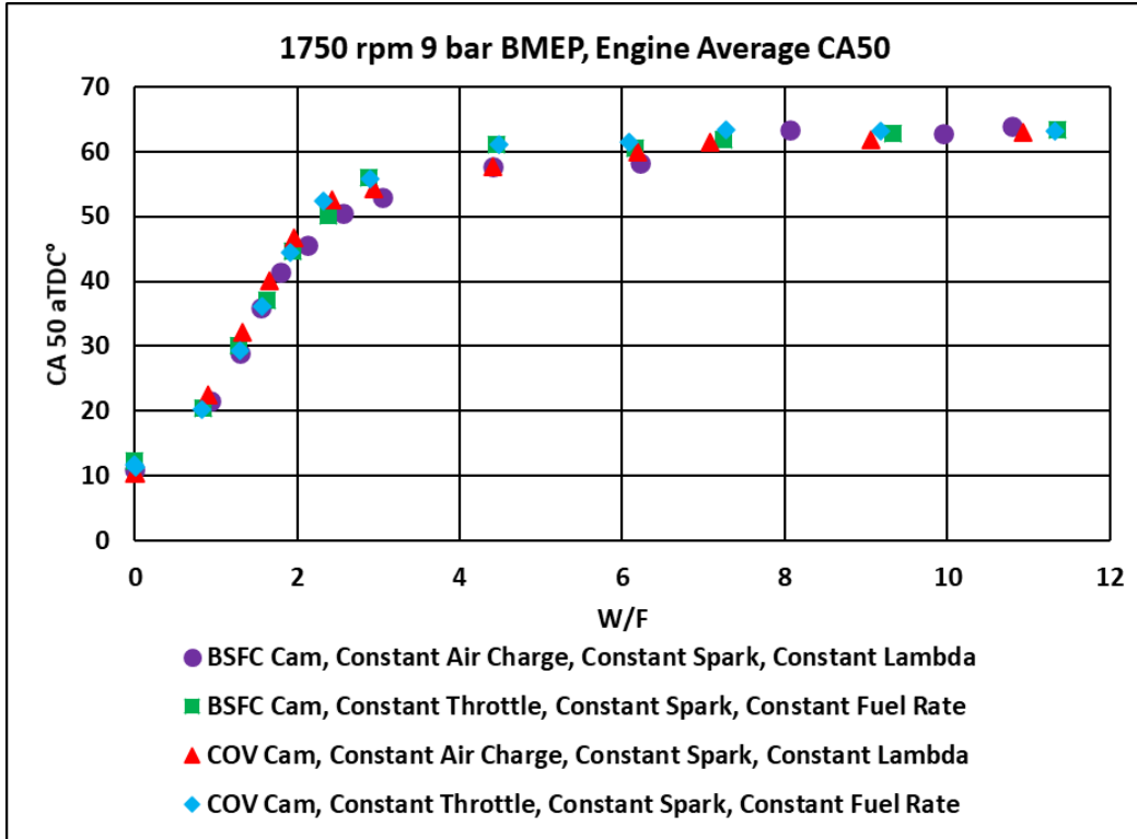
Figure 33 1750 RPM test point atomized spray CA50 plot
